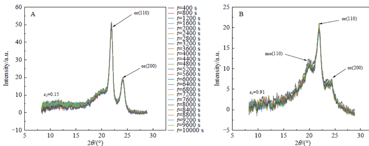
Fig. 6 One-dimensional WAXD curves of the sample during fatigue testing at pre-strains of (A) 0.15 and (B) 0.91
